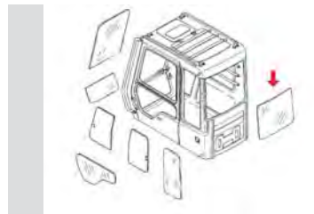
4602569 Excavator Rear Windowpane
